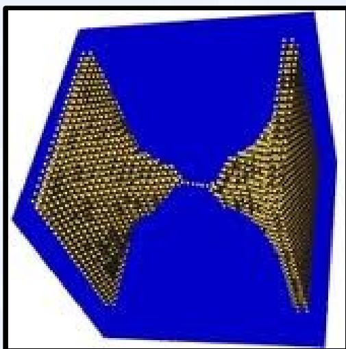
Break junction
