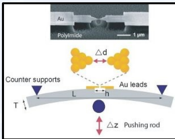
Break junction
