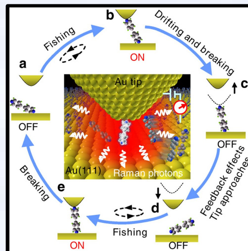
STM
